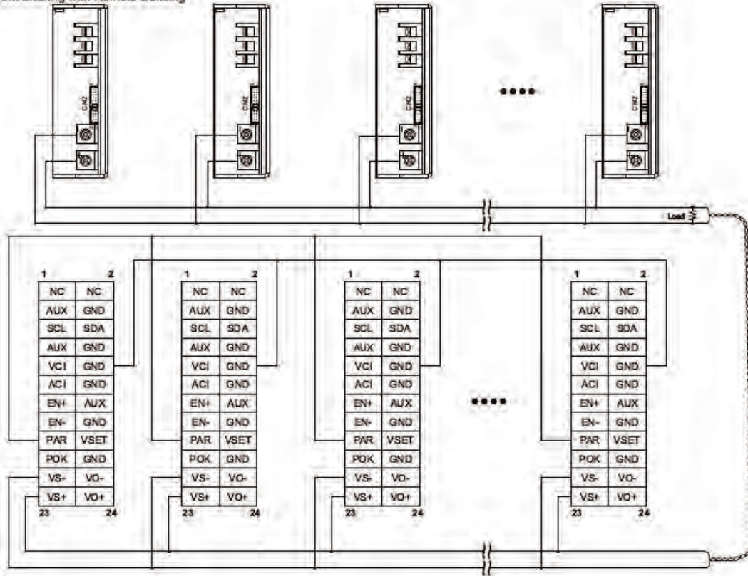
4. Current Sharing with Local Sensing
