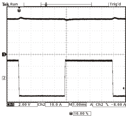
SM18-50 with Power Sink Option Current - 15 A means the load delivers 15 A to the power supply (sink operation)
