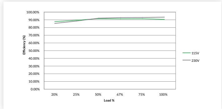
Figure 4 GCS180PS24
