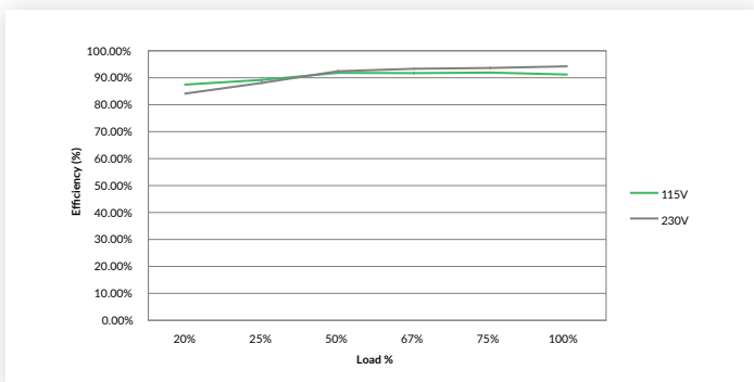
Figure 5 GCS180PS48
