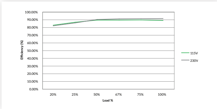
Figure 3 GCS180PS12
