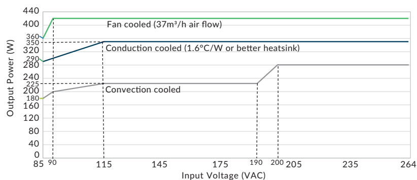
Input derating curve
