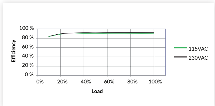
Figure 4 GSP750PS24
