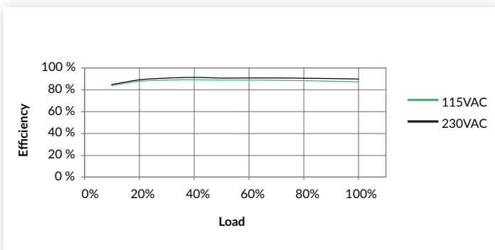
Figure 3 GSP750PS12
