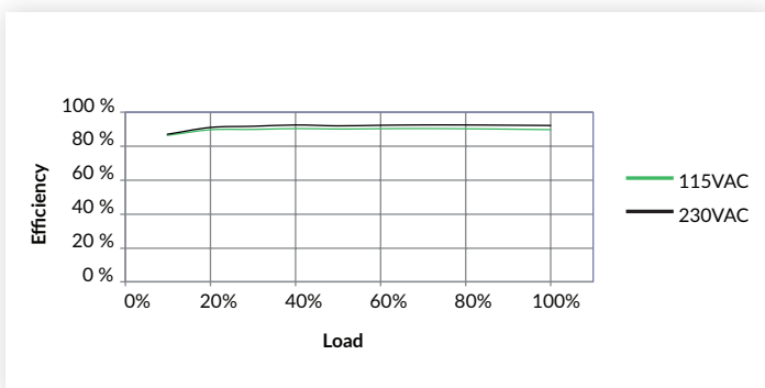
Figure 5 GSP750PS48
