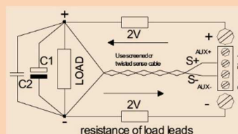
Remote Sensing (twist wires)
